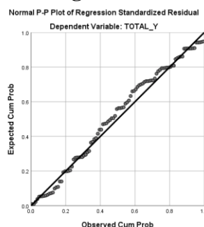
Grafik 3.4 Normal P-Plot of Regression Standardized Residual
